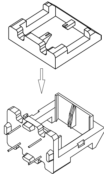
PART P-2803
